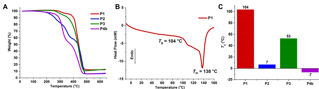
Figure 7. Thermal properties of depolymerizable polyheptenamers. (A) Thermogravimetric analysis of functional polyheptenamers (P1–P4b). (B) Differential scanning calorimetry (DSC) thermogram of P1. (C) Glass transition temperatures of P1–P4b determined by DSC.
